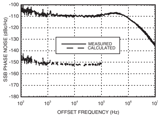
[1] Phase Noise Floor remains constant beyond 100 kHz offset frequency. Measured phase noise using Agilent 5500 with 2 unit measurement technique and corresponding calculated phase noise floor.
