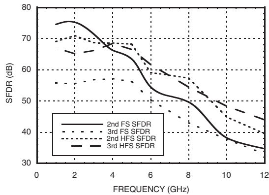
Hold-Mode SFDR vs. Frequency & Input Power @ f_{clk} = 1 \text{ GHz} @ +6 \text{ dBm}
