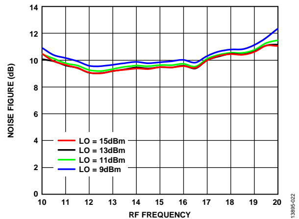
Figure 22. Noise Figure vs. RF Frequency at Various LO Power Levels, TA = 25°C
