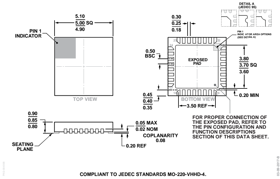
Figure 37. 32-Lead Lead Frame Chip Scale Package [LFCSP] 5 mm x 5 mm and 0.85 mm Package Height (HCP-32-1) Dimensions shown in millimeters
