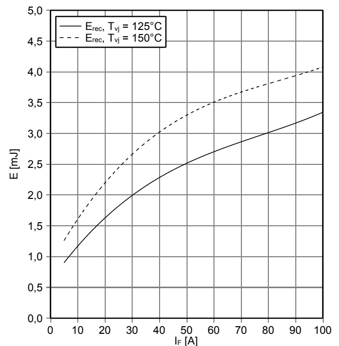
Schaltverluste Diode, D1 / D4 (typisch) switching losses Diode, D1 / D4 (typical) E_{rec} = f(I_F) R_{Gon} = 5.1\ \Omega , V_{CE} = 400\text{ V}
