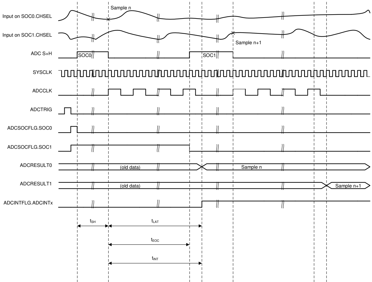
Figure 7-35. ADC Timings
