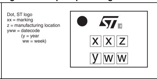
Figure 27. Flip-Chip marking
