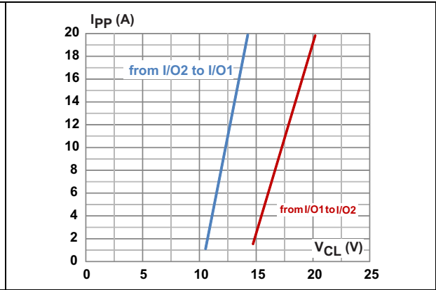
Figure 10. TLP measurements
