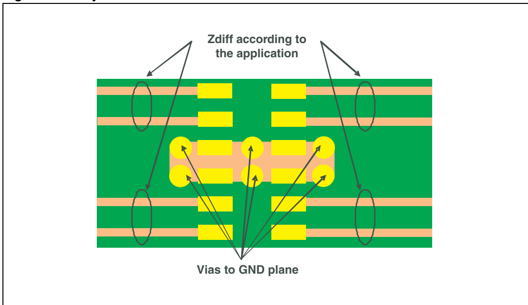
Figure 20. Layout recommendation
