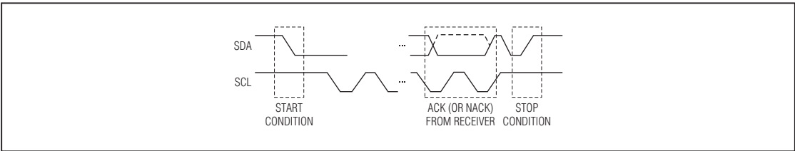
Figure 6. Start, Stop, and ACK Signals
