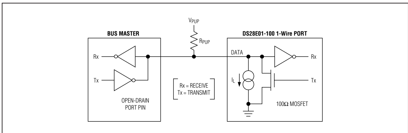
Figure 9. Hardware Configuration
