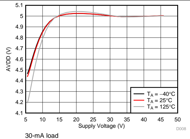
Figure 10. AVDD Regulator
