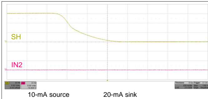
Figure 54. SH Fall Time
