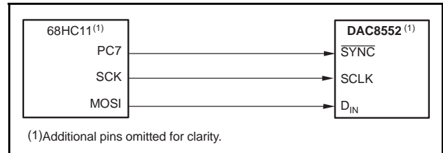
Figure 48. DAC8552 to 68HC11 Interface
