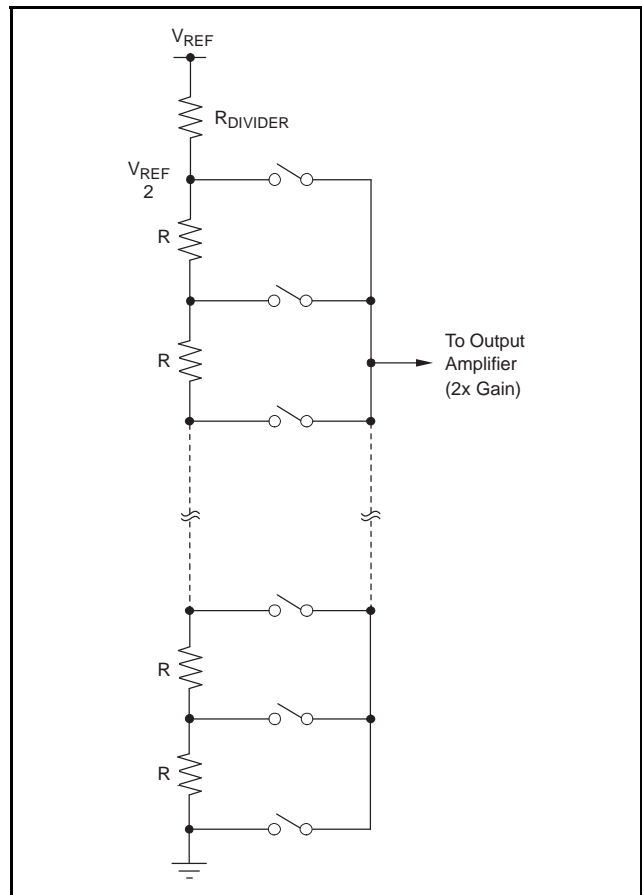
Figure 42. Resistor String
