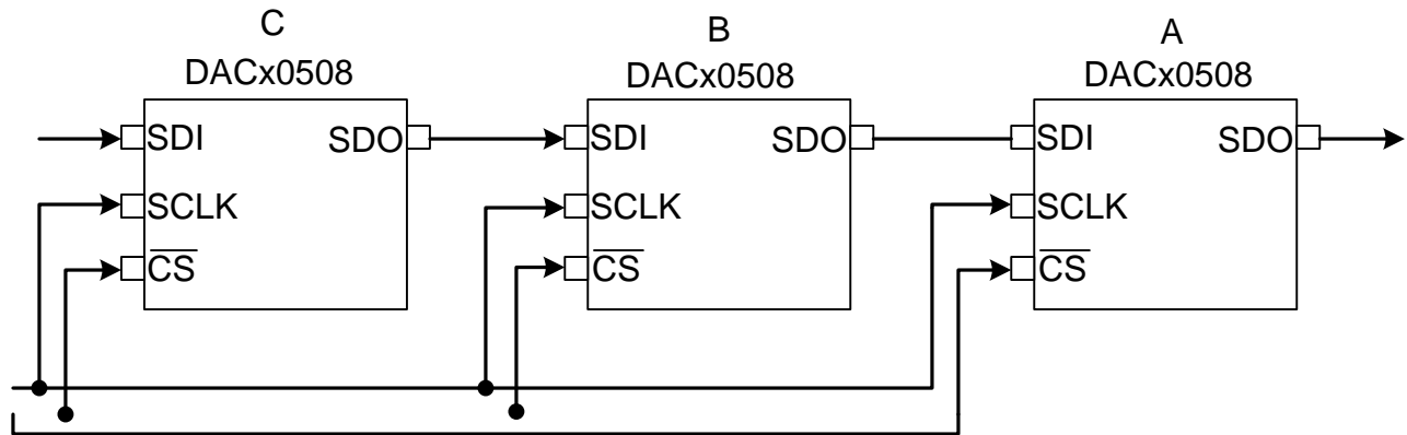
Figure 61. Daisy-Chain Layout
