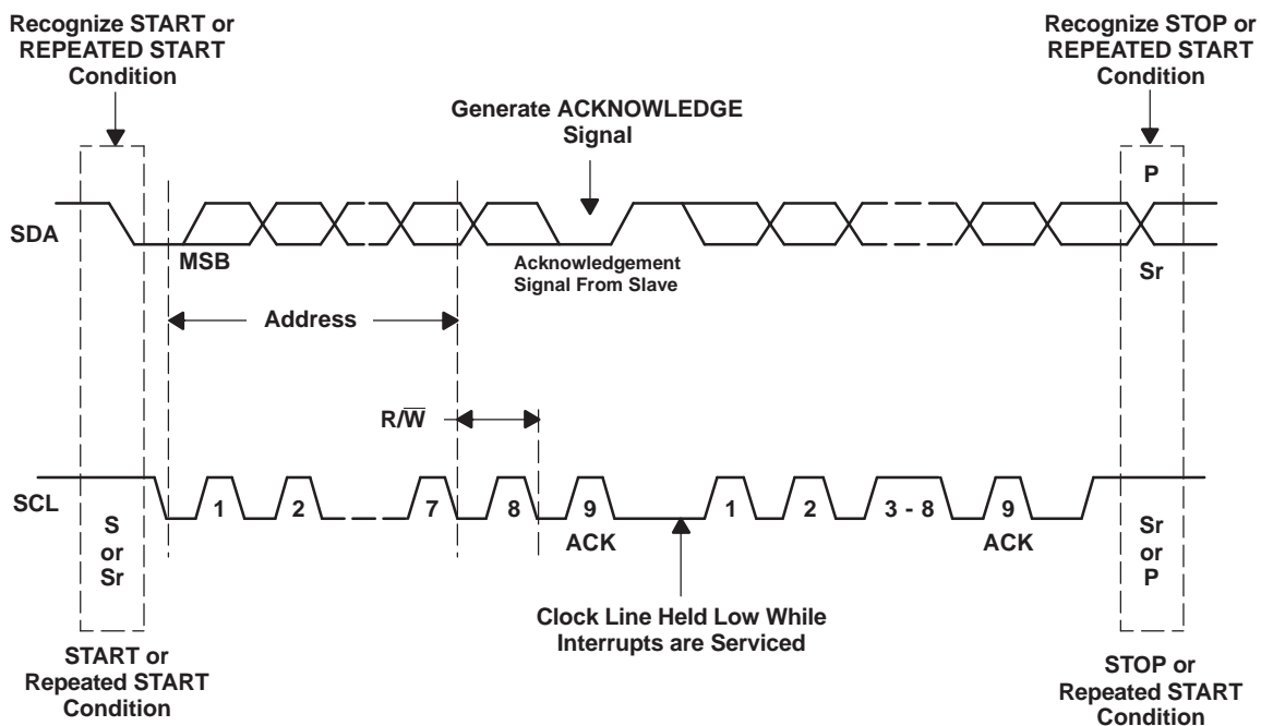
Figure 44. Bus Protocol
