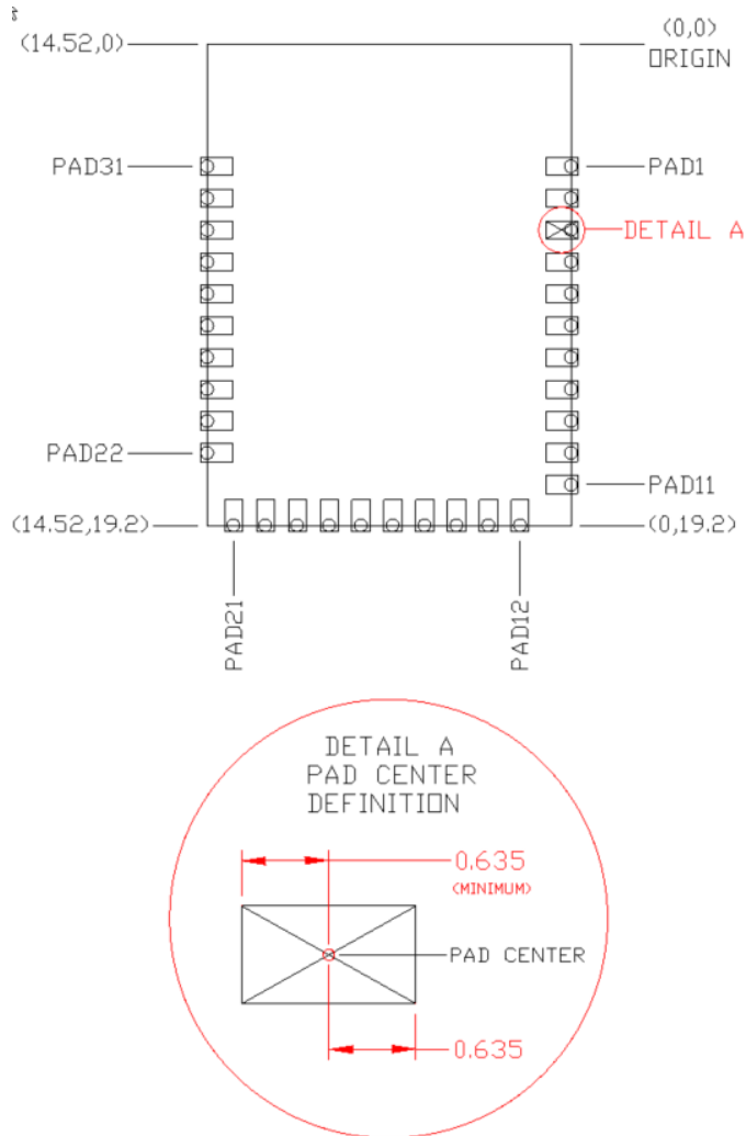
Figure 6. Solder Pad Reference Location
