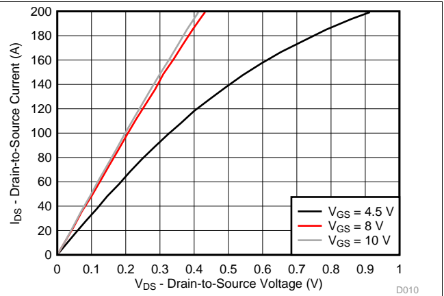
Figure 8. MOSFET Saturation Characteristics
