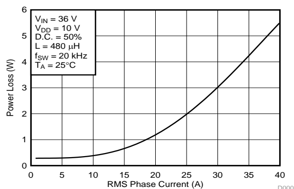
Power Loss vs Output Current
