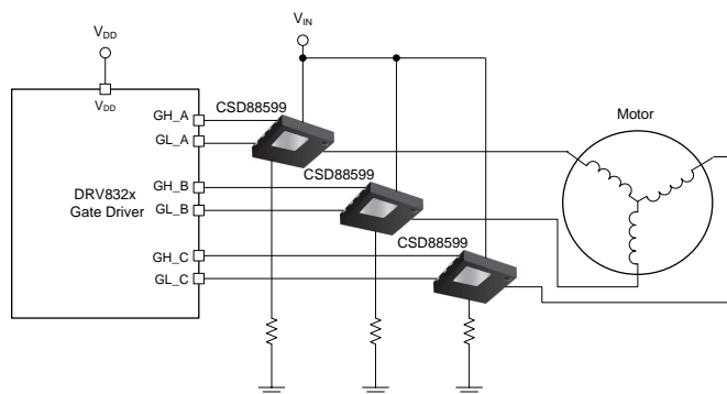
Typical Circuit
