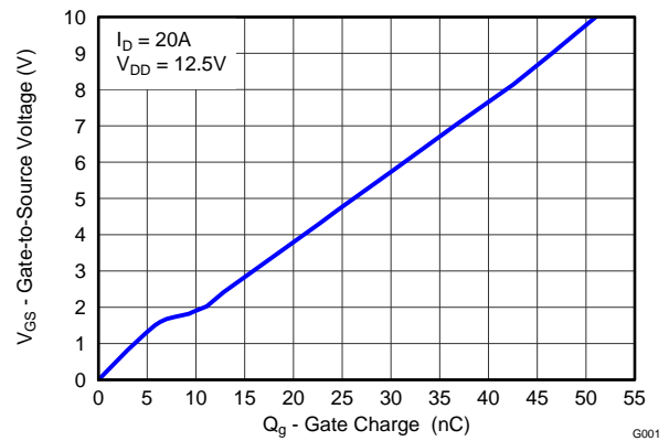
Figure 15. Sync MOSFET Gate Charge
