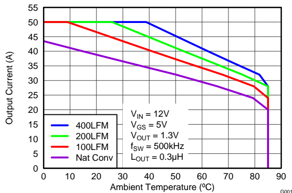
Figure 4. Safe Operating Area – PCB Horizontal Mount (1)
