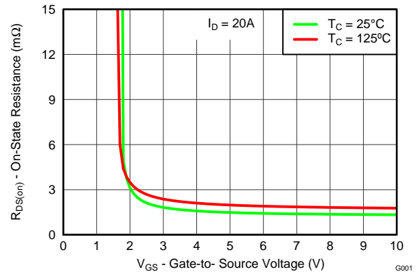
Figure 21. Sync MOSFET R DS(on) vs V GS
