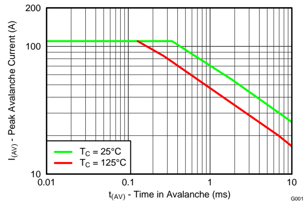
Figure 27. Sync MOSFET Unclamped Inductive Switching
