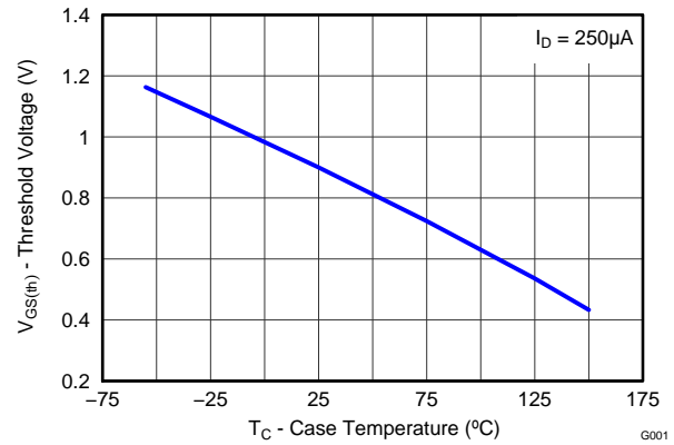
Figure 19. Sync MOSFET V GS(th)
