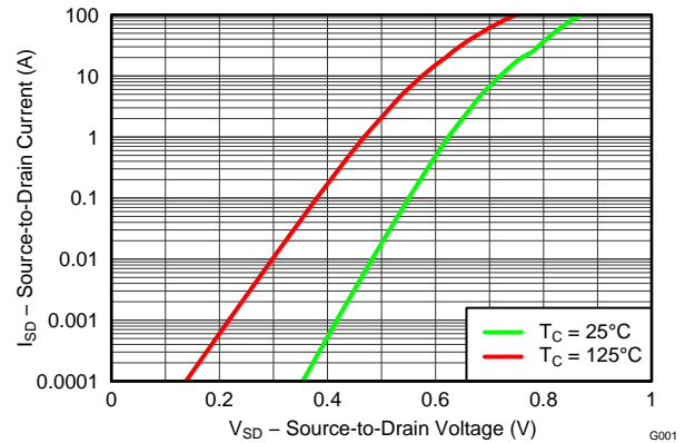
Figure 25. Sync MOSFET Body Diode
