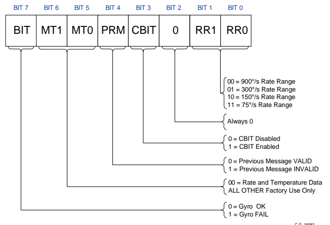
Figure 7.10 Status Byte Format
