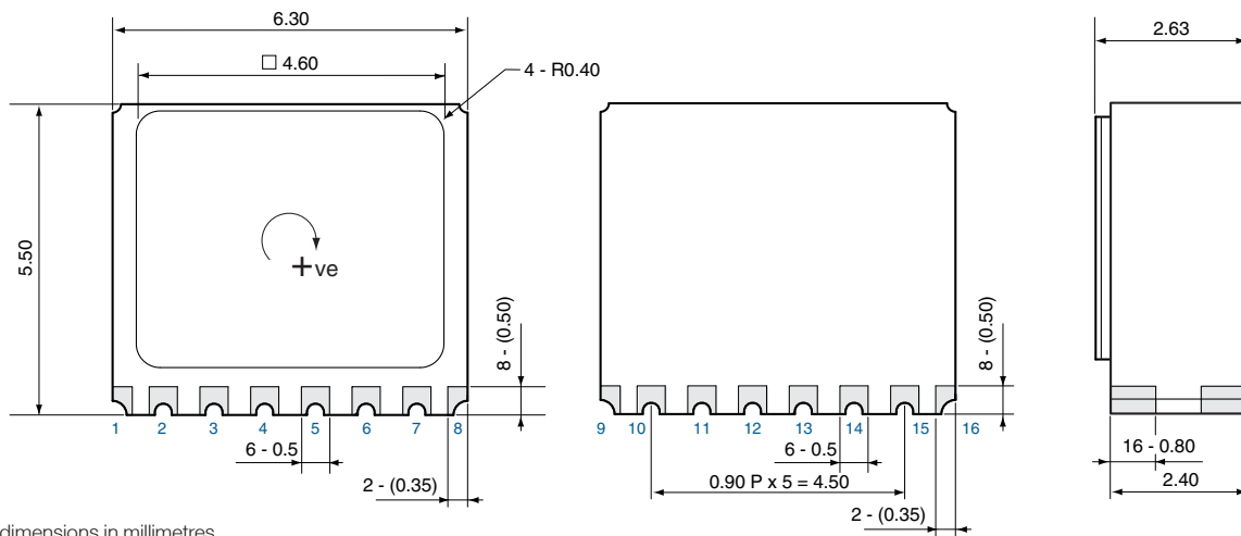
Figure 1.2 CRM200 Overall Dimensions
