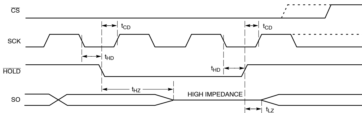
Figure 11. HOLD Timing
