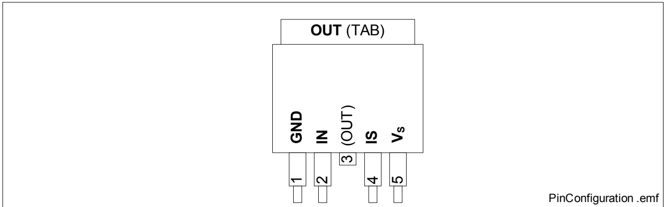
Figure 2 Pin Configuration
