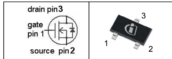
PG-SC-59
