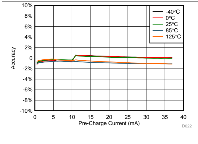
Figure 11. Pre-Charge Accuracy vs Pre-Charge Current
