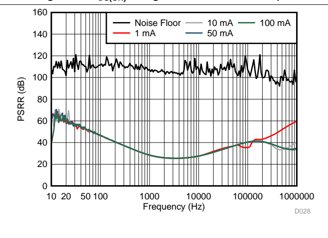
Figure 14. LS/LDO PSRR vs Frequency
