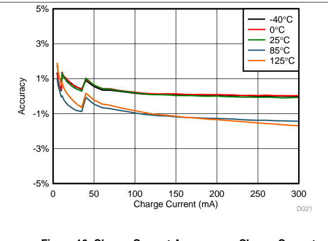
Figure 10. Charge Current Accuracy vs Charge Current
