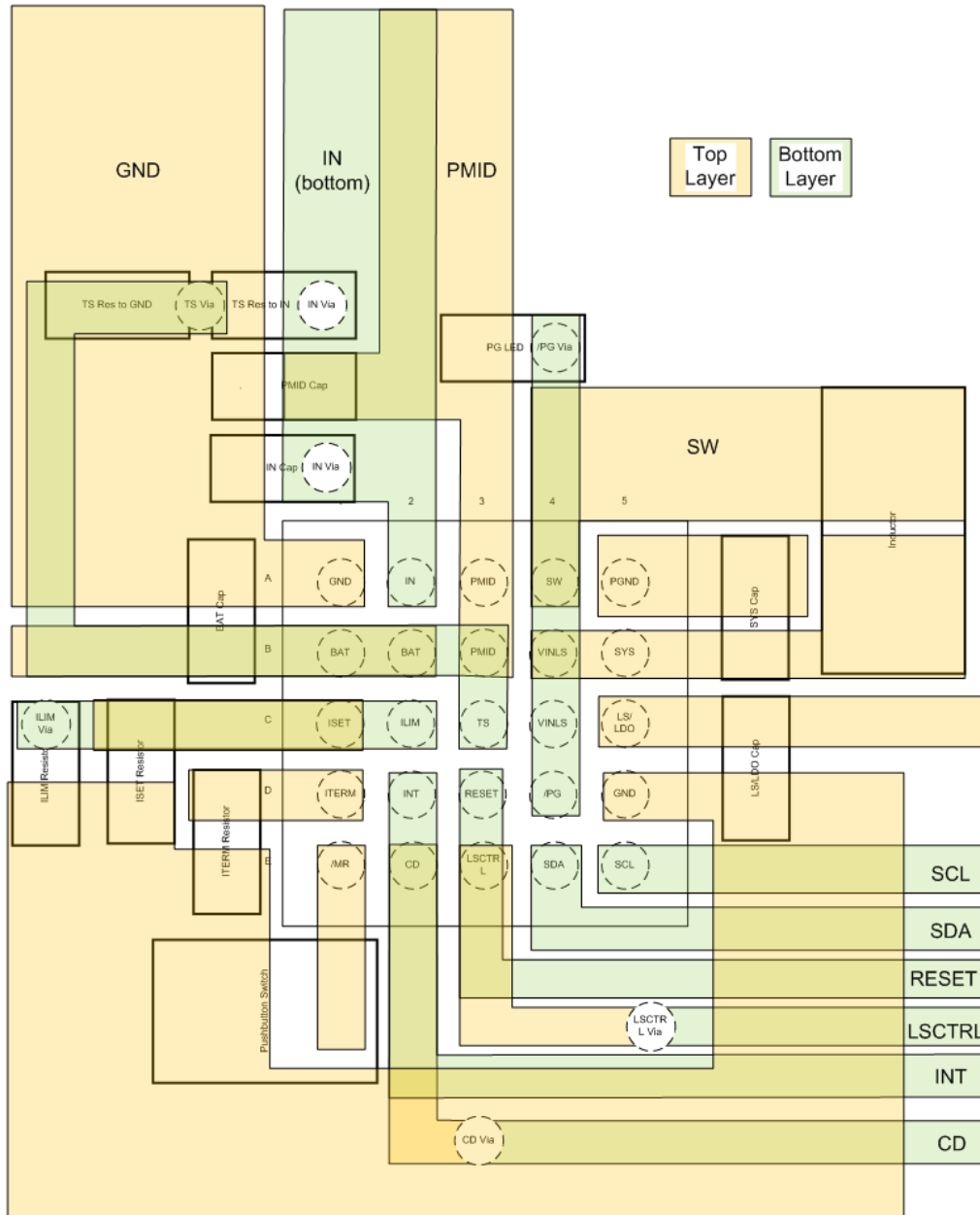
Figure 105. BQ25121A Layout
