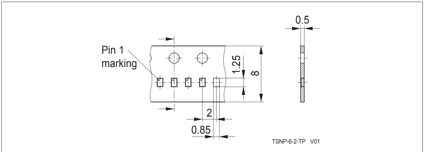
Figure 6: Tape Drawing for TSNP-6-2
