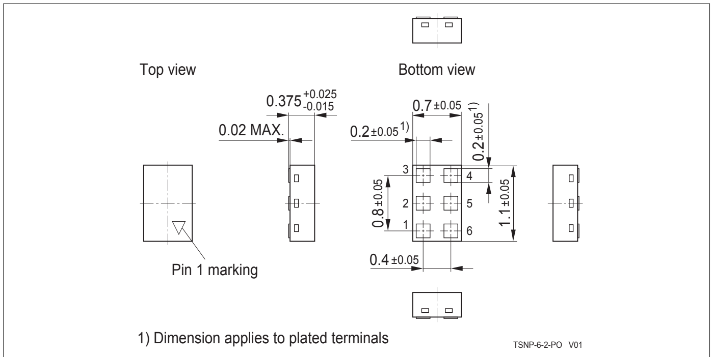
Figure 3: Package Outline
