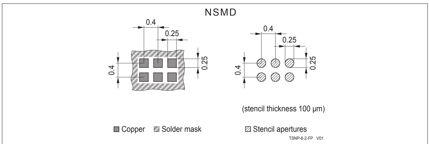
Figure 4: Footprint
