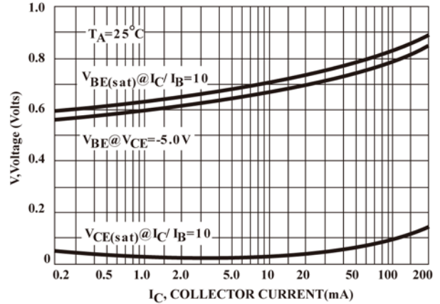
Figure 8. "ON" Voltage
