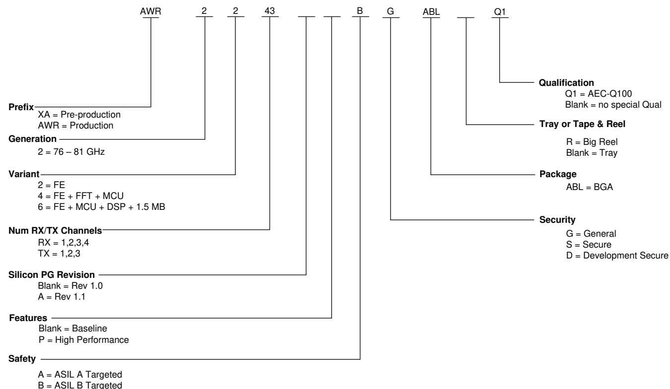
Figure 12-1. Device Nomenclature
