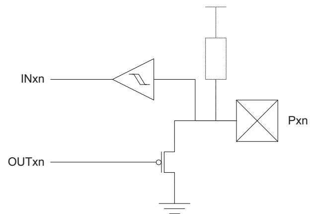
Figure 16-6. I/O configuration - Wired-AND with optional pull-up.
