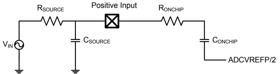
Figure 7-7. ADC Input
