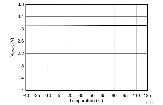
Figure 5. Common-Mode Overvoltage Detection Level vs Temperature
