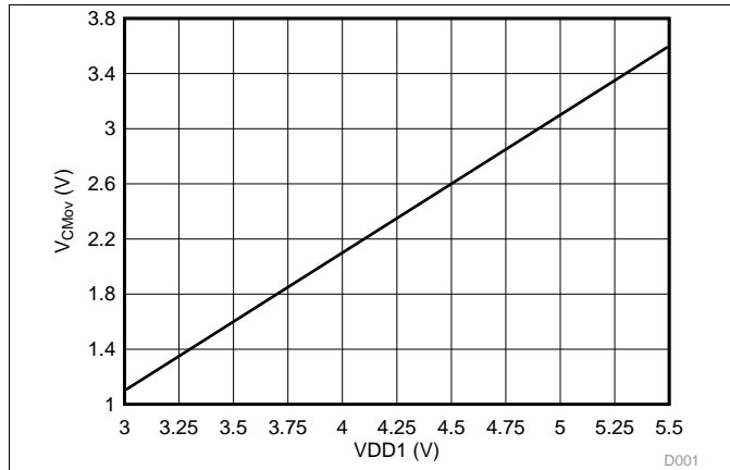
Figure 4. Common-Mode Overvoltage Detection Level vs High-Side Supply Voltage
