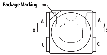
Figure 11b. Component Axis for Radiation Pattern
