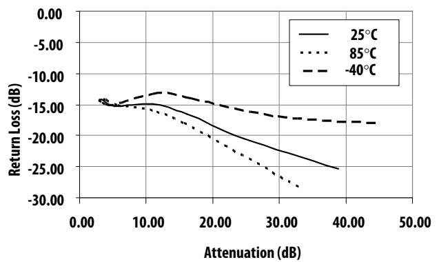
Figure 27. Return loss vs Attenuation vs Temperature at 1900MHz
