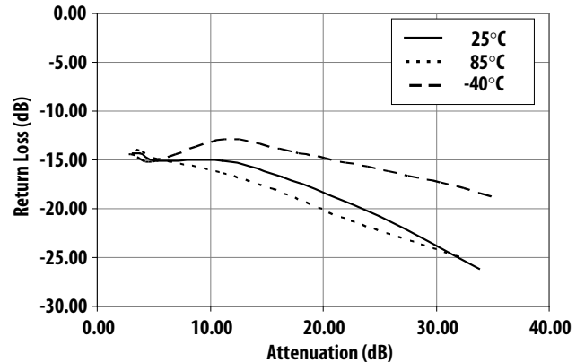
Figure 11. Return loss vs Attenuation vs Temperature at 1900MHz
