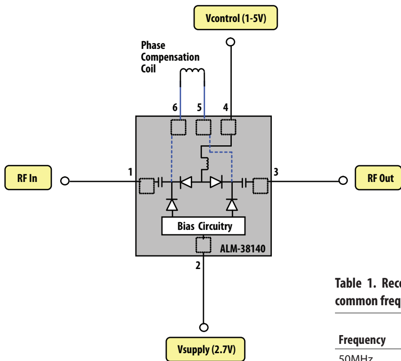
Figure 32. Simplified Schematic
