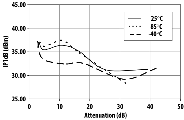
Figure 12. Input P1dB vs Attenuation vs Temperature at 900MHZ
