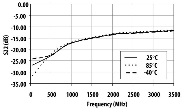
Figure 21. S22 (Return Loss) at Vctrl=5V vs Frequency vs Temperature
