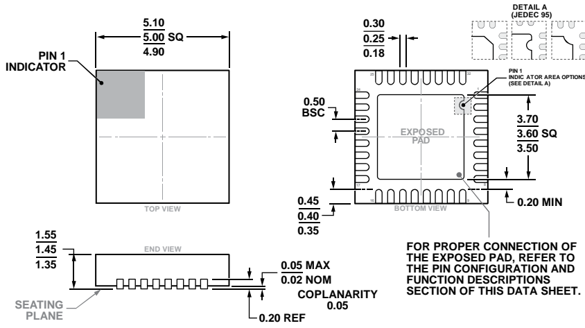
Figure 40. 32-Lead Lead Frame Chip Scale Package [LFCS] 5 mm × 5 mm Body and 1.45 mm Package Height (CP-32-17)
