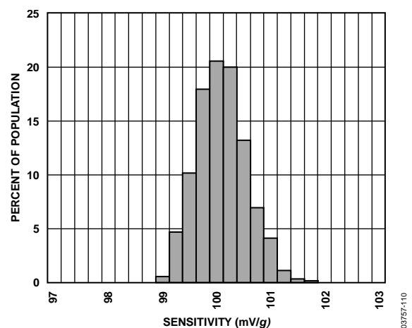
Figure 30. Y-Axis Sensitivity at 25°C
