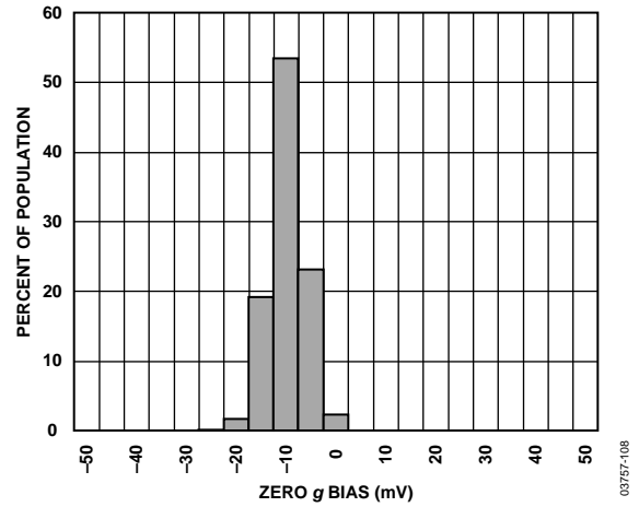
Figure 28. Y-Axis Zero g Bias Deviation from Ideal at 25°C
