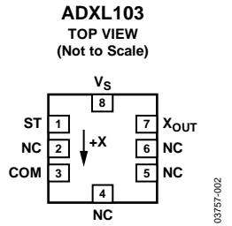
Figure 3. ADXL103 Pin Configuration
