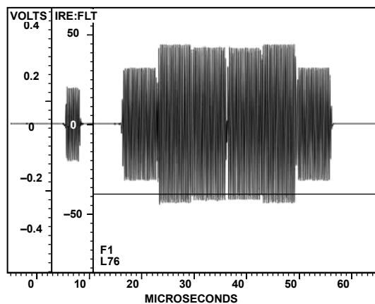
Figure 132. NTSC Chroma
