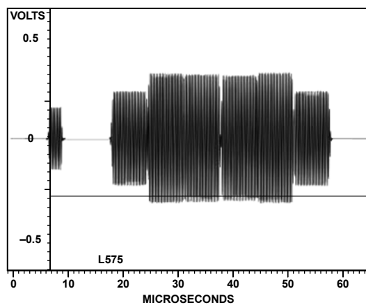
Figure 135. PAL Chroma
