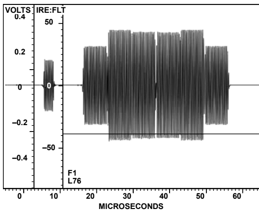
Figure 130. NTSC Chroma
