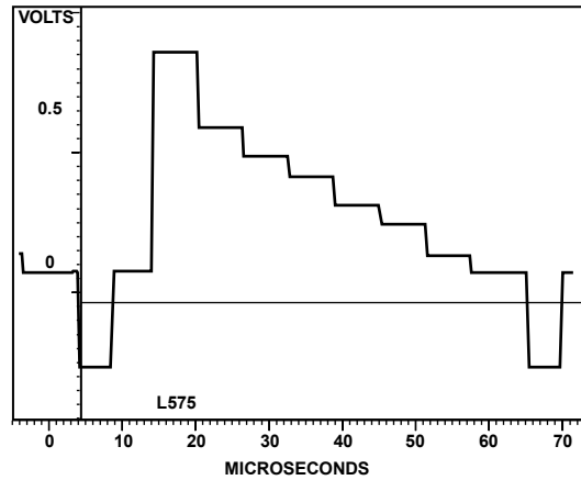
Figure 132. PAL Luma
