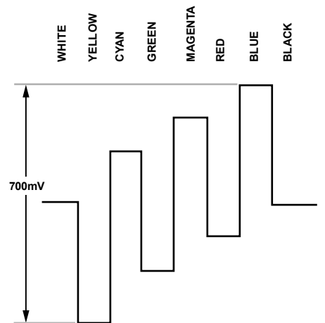
Figure 119. Pb Levels—PAL
