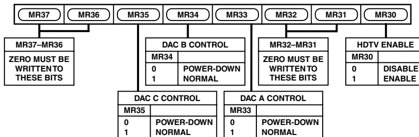
Figure 54. Mode Register 3
