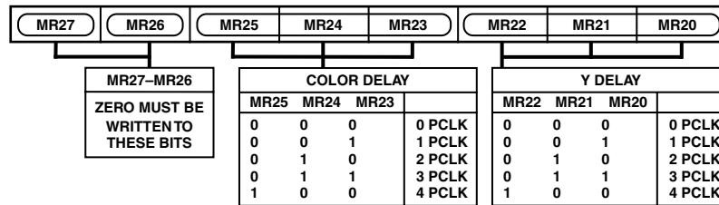
Figure 53. Mode Register 2
