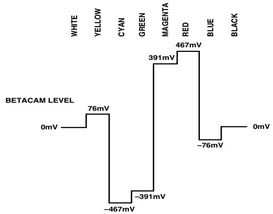
Figure 125. NTSC 100% Color Bars with Pedestal V
