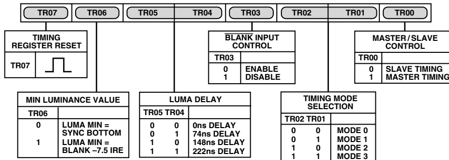
Figure 66. Timing Register 0
