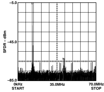
TPC 9. Dual-Tone SFDR @ f_{CLOCK} = 140\text{ MHz} ( f_{OUT1} = 13.5\text{ MHz} , f_{OUT2} = 14.5\text{ MHz} )
