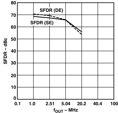
TPC 11. SFDR vs. f_{OUT} @ f_{CLOCK} = 50\text{ MHz} (Single-Ended and Differential)
