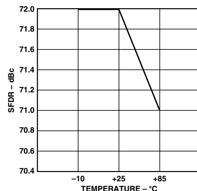
TPC 3. SFDR vs. Temperature @ f_{CLOCK} = 50\text{ MHz} ( f_{OUT} = 1\text{ MHz} )
