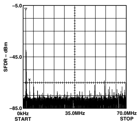
TPC 7. Single-Tone SFDR @ f_{CLOCK} = 140\text{ MHz} ( f_{OUT} = 2\text{ MHz} )
