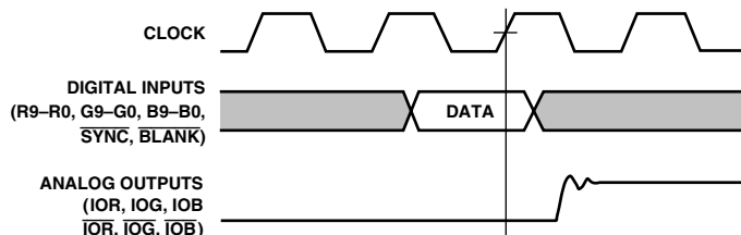
Figure 2. Video Data Input/Output
