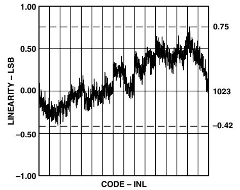
TPC 15. Typical Linearity
