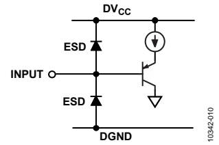
Figure 27. Logic Input
