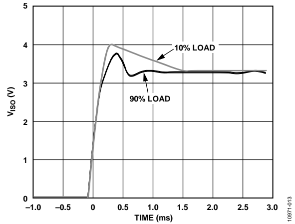
Figure 13. Typical Output Voltage Start-Up Transient at 10% and 90% Load, V_{ISO} = 3.3\text{ V}
