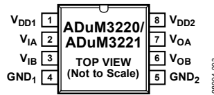
Figure 4. Pin Configuration
