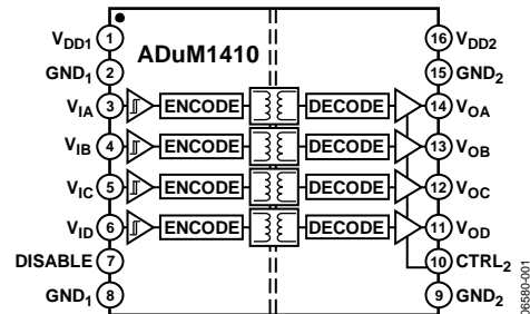
Figure 1. ADuM1410
