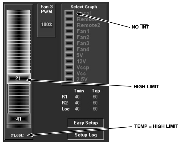
Figure 30. Temperature = High Limit: No \overline{\text{INT}}
