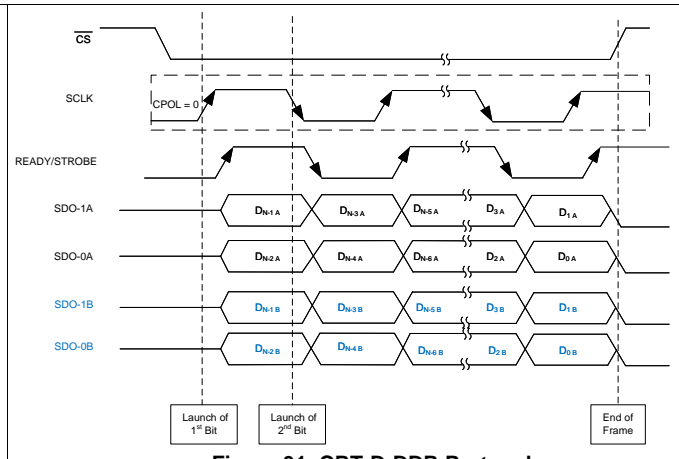
Figure 31. CRT-D-DDR Protocol
