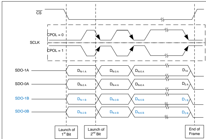
Figure 21. SPI-00-D-SDR and SPI-10-D-SDR Protocols
