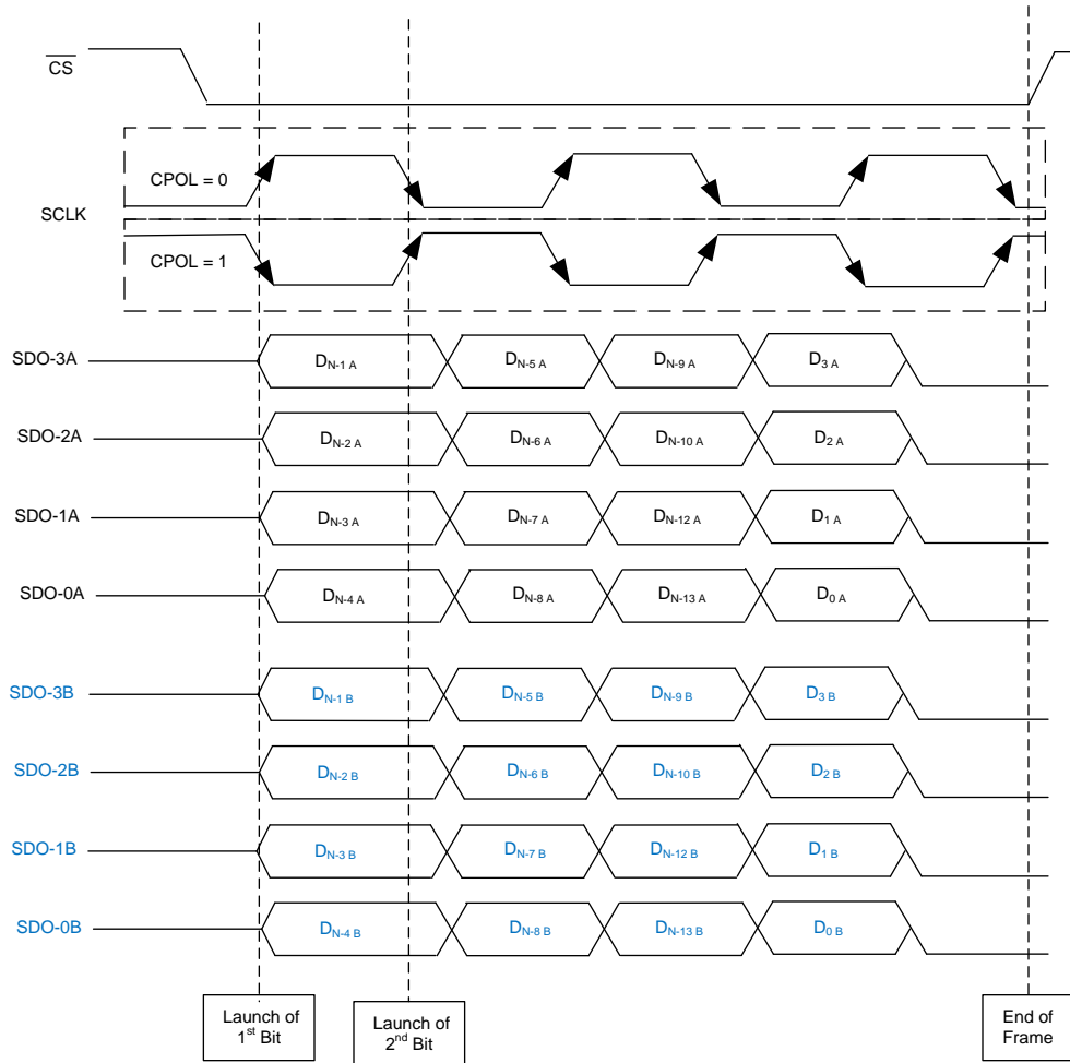
Figure 27. SPI-01-Q-DDR and SPI-11-Q-DDR Protocols
