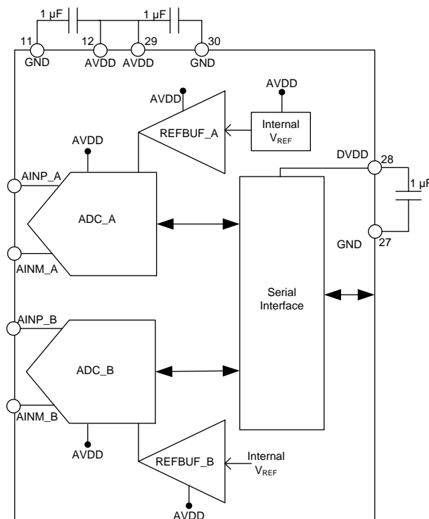
Figure 53. Power-Supply Decoupling
