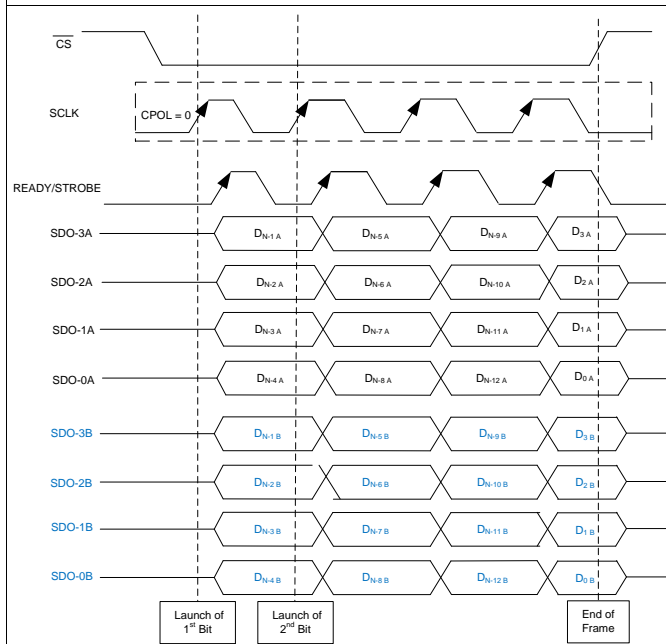
Figure 32. CRT-Q-SDR Protocol
