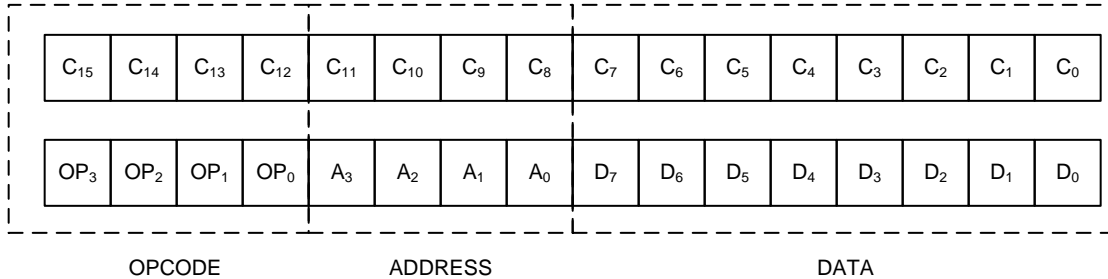
Figure 40. Command Frame C[15:0]
