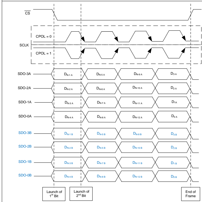
Figure 23. SPI-00-Q-SDR and SPI-10-Q-SDR Protocols
