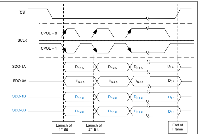
Figure 22. SPI-01-D-SDR and SPI-11-D-SDR Protocols
