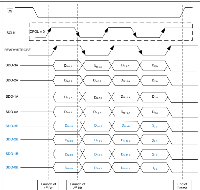
Figure 33. CRT-Q-DDR Protocol
