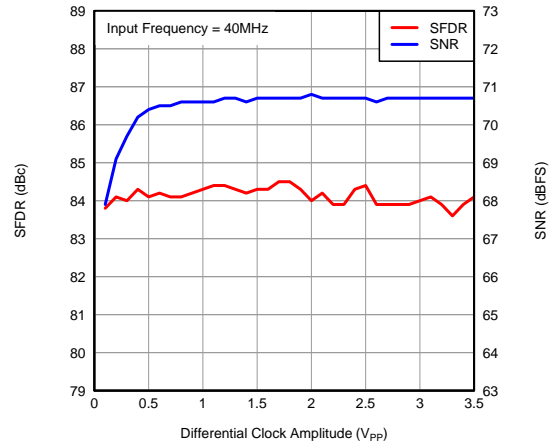
Figure 22. Performance Across Input Clock Amplitude
