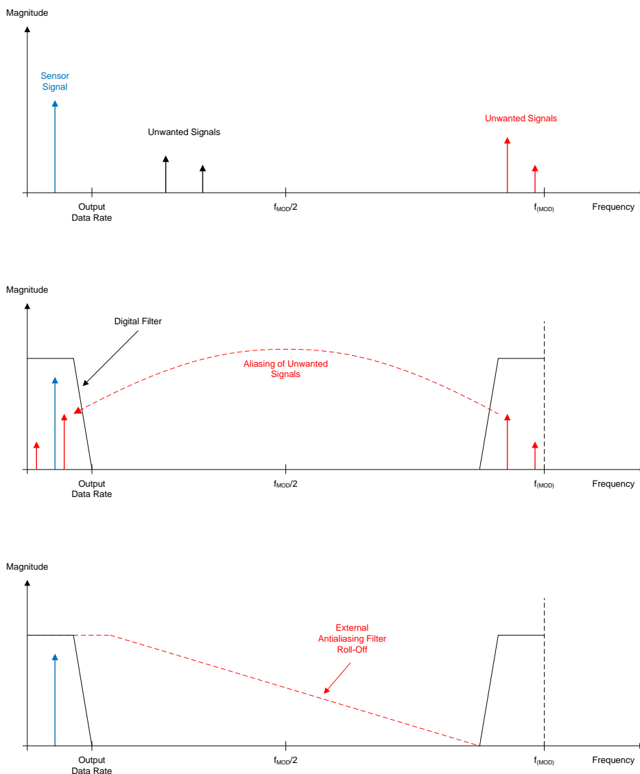
Figure 35. Effect of Aliasing
