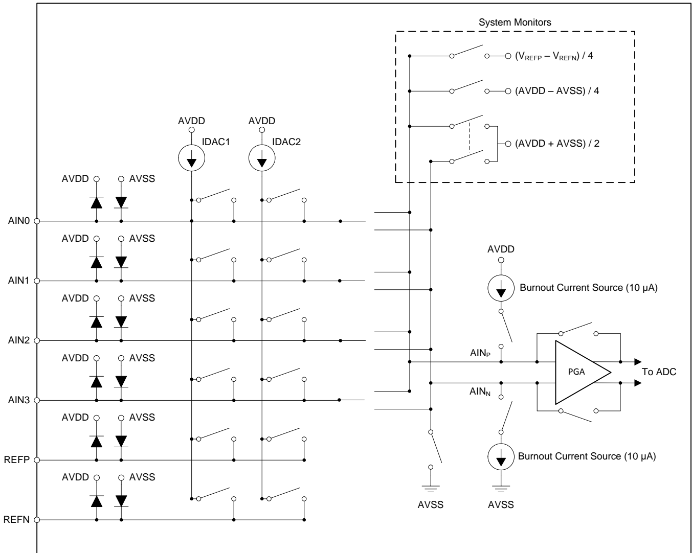
Figure 7. Analog Input Multiplexer
