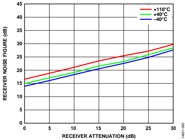
Figure 124. Receiver Noise Figure vs. Receiver Attenuation, 3500 MHz LO, 100 MHz Bandwidth, 153.6 MSPS Sample Rate, 50 MHz Integration Bandwidth (Includes 1 dB Matching Circuit Loss)
