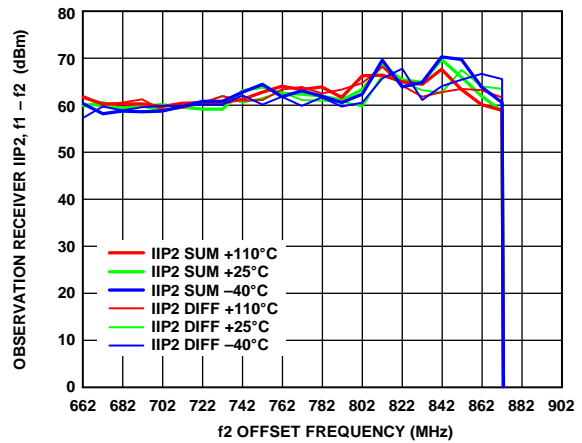
Figure 115. Observation Receiver IIP2, f1 - f2 vs. f2 Offset Frequency, LO = 650 MHz, Tone 1 = 652 MHz, Tone 2 = Swept at -19 dBm Each, Observation Receiver Attenuation = 0 dB
