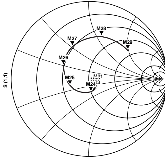
Figure 265. Transmitter Output Impedance Series Equivalent Differential Impedance (SEDZ)
