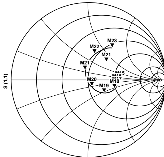
Figure 266. Observation Receiver Input Impedance SEDZ
