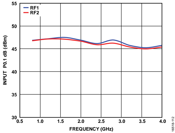
Figure 11. Input 0.1dB Power Compression ( P_{0.1\text{ dB}} ) vs. Frequency, V_{DD} = 5\text{ V}
