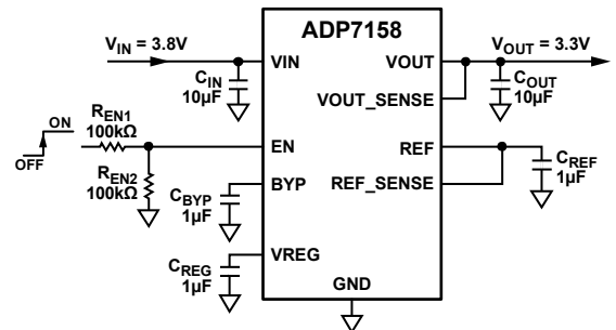
Figure 51. Typical EN Pin Voltage Divider
