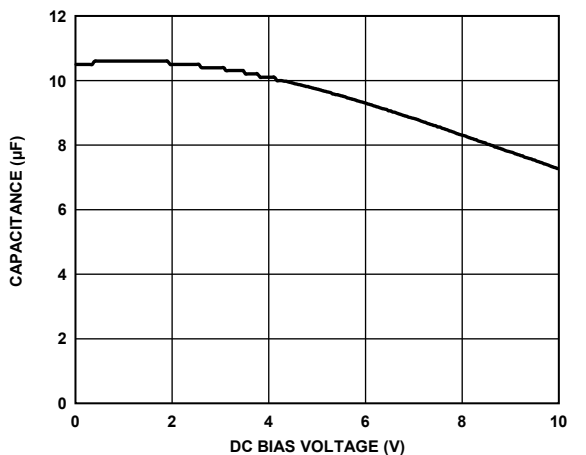
Figure 46. Capacitance vs. DC Bias Voltage
