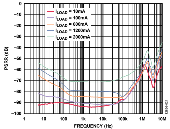
Figure 21. Power Supply Rejection Ratio (PSRR) vs. Frequency at Various Loads, V_{OUT} = 3.3V , V_{IN} = 4.0V
