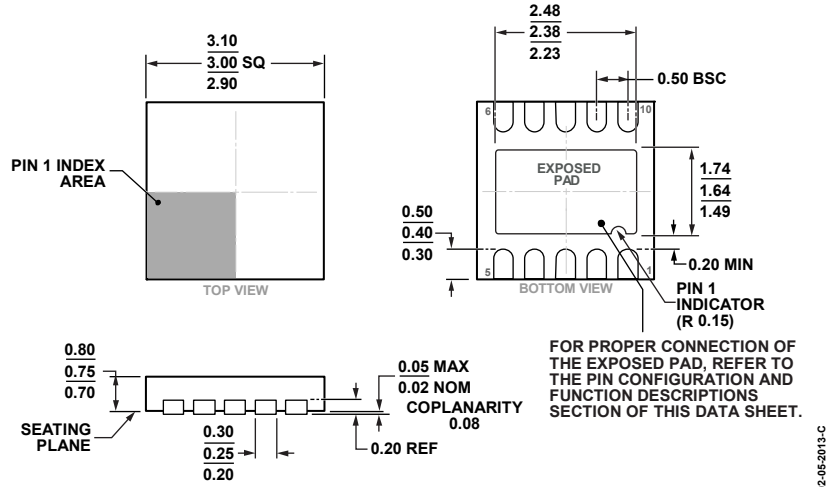
Figure 64. 10-Lead Lead Frame Chip Scale Package [LFCSP] 3 mm x 3 mm Body and 0.75 mm Package Height (CP-10-9) Dimensions shown in millimeters
